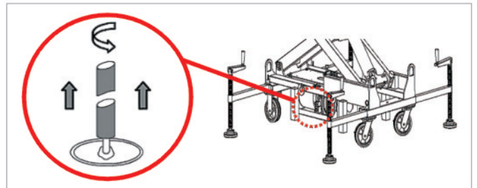
Manual Lowering Valve in case of power failure.
