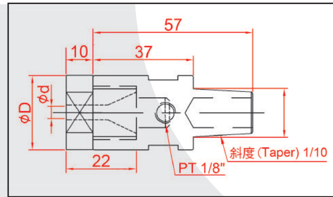
螺帽電極-黑鋼心用 Electrode for Steel pins
