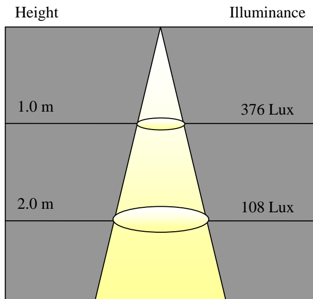
Average Illuminance Figure
