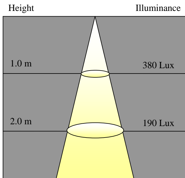
Average Illuminance Figure
