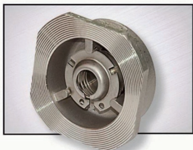
Spring Loaded Wafer Check Valve
