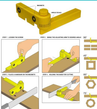
Hand Saw Mitre Gauge
