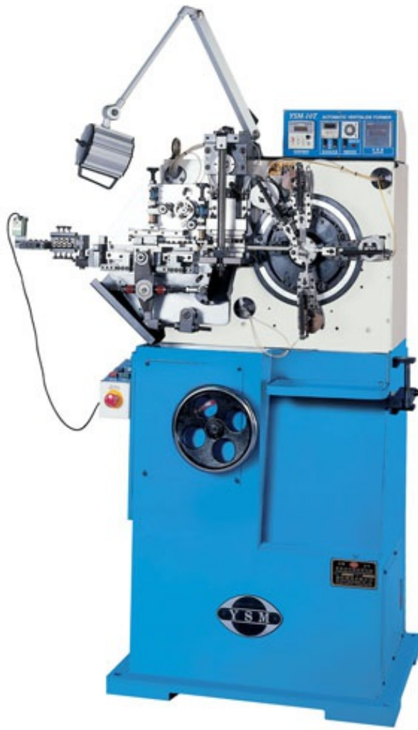
Strip & Wire Forming Machine
