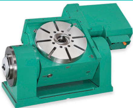
Manual Tilting CNC Rotary Table
