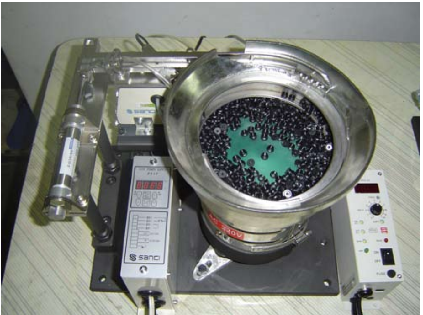
Vibrating material feeder
