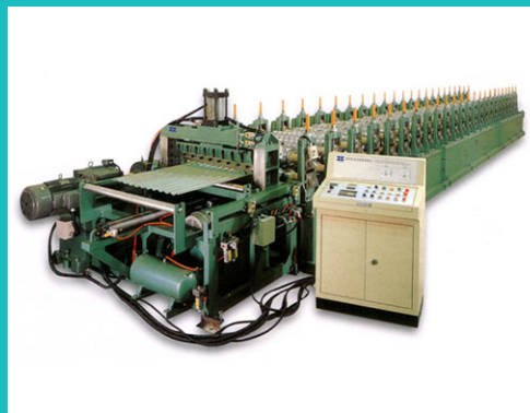
Fully Automatic Corrugated Roofing Sheet Cold-Roll-Forming Machine (NC or Air Controlled)
