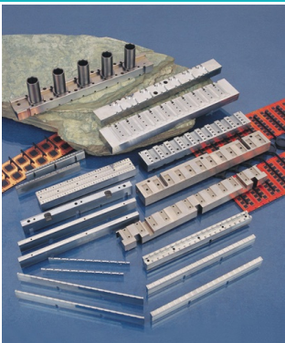
Cavity Bar
