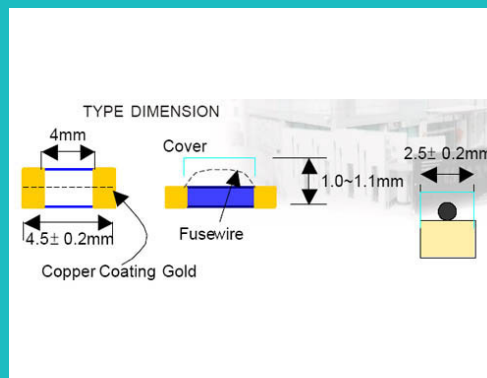
SMD Fuse
