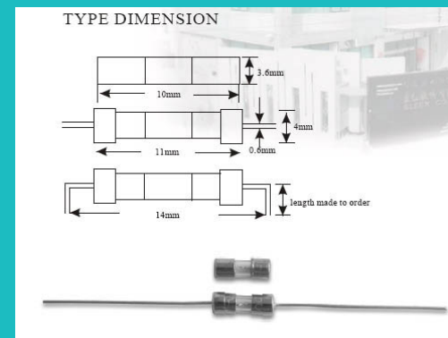
Micro Fuse
