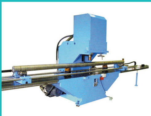
Digital Press Straightening Machine
