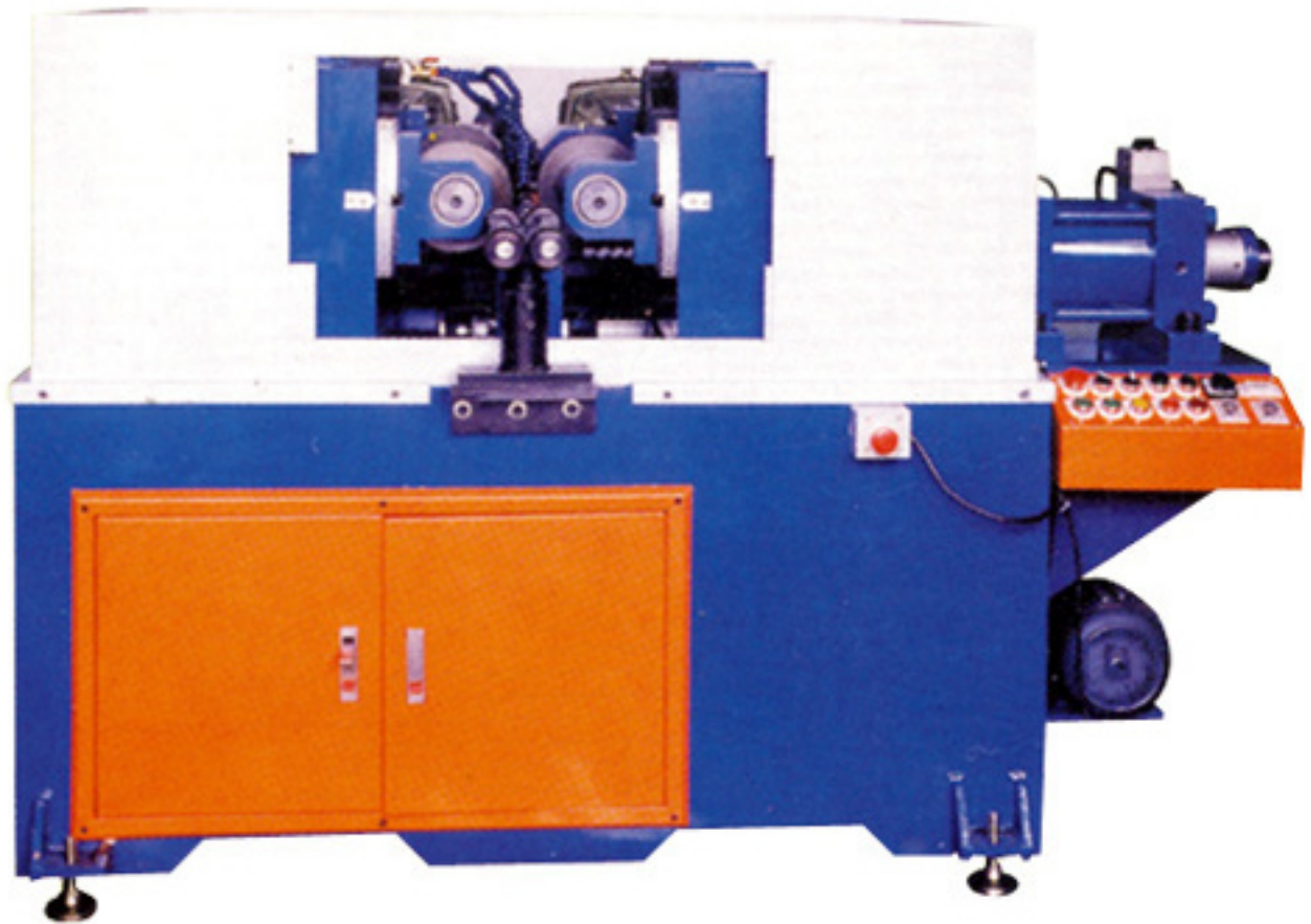
Through-Feed Straightening Machine
