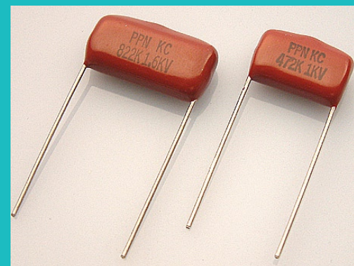
PPN Polypropylene Film Foil Capacitor (Noninductive)
