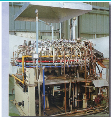
24HD Tubulating Machine
