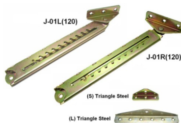
Lid Support
