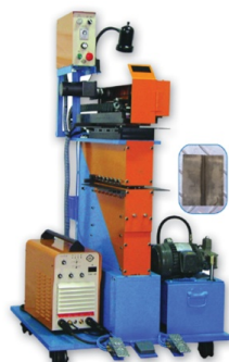
Steel Coil Joint Welding Machine
