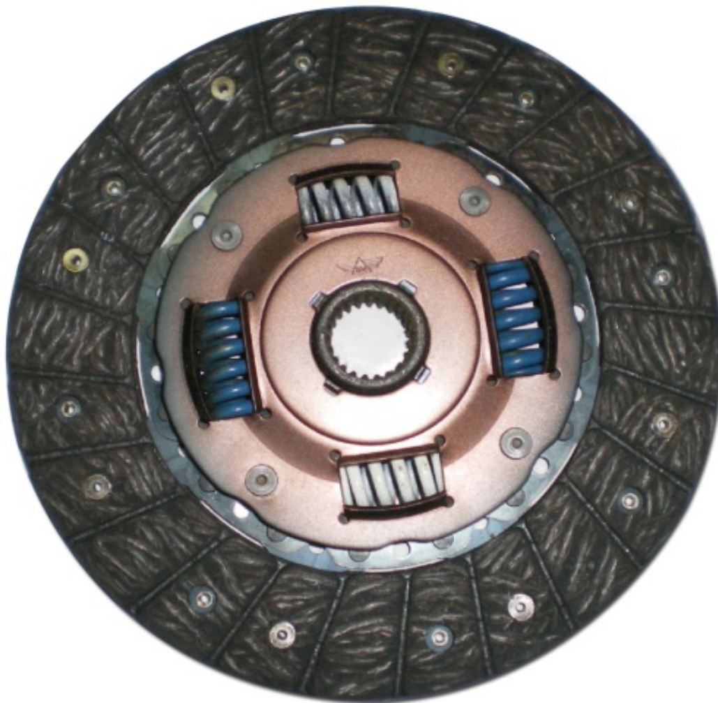
Clutch Plates
