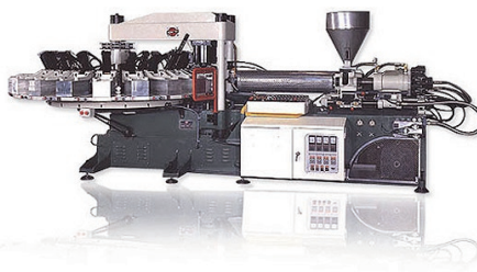
Rotary Type Automatic Air Blowing Plastic Shoes Injection Molding Machine
