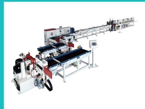
Finger Joint
