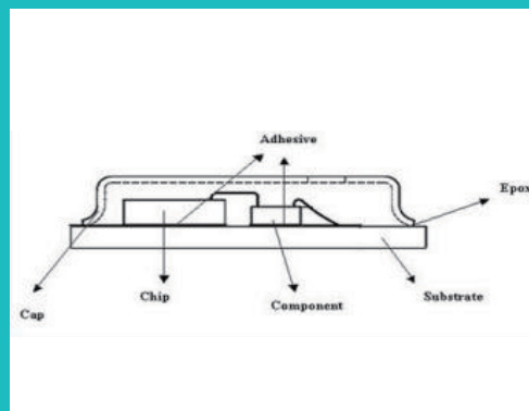
LGA, MEMS micro phone
