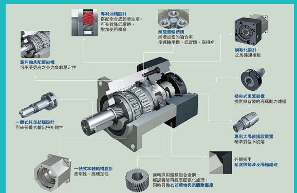
Reducer product structure
