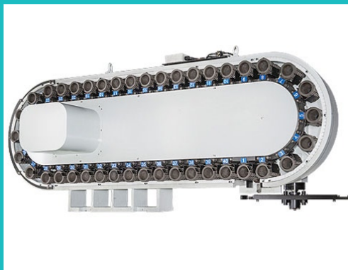
VERTICAL SERIES CHAIN-TYPE MAGAZINE
