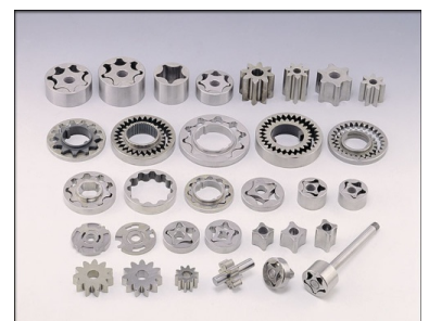
Oil-pump gears
