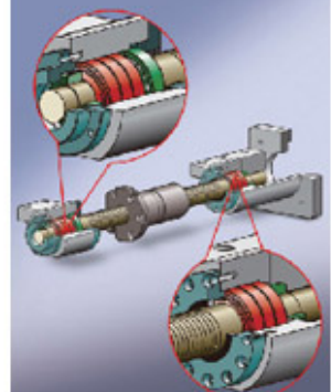
Enhanced Screw Pretension Design
