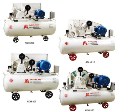
Air Compressors Two Stage Middle Pressure Type
