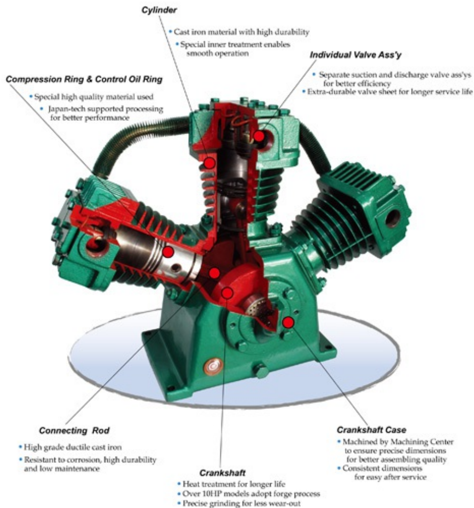
Air Compressors OTTOTEK Compressor Features
