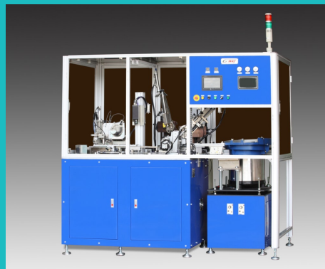
Oil Seal Trimming, Spring Loading and Dimension Measuring Machine
