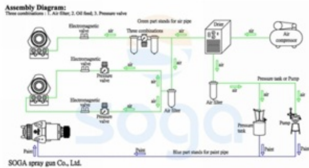
Automatic spray gun /Auto spray gun of high efficiency for robot
