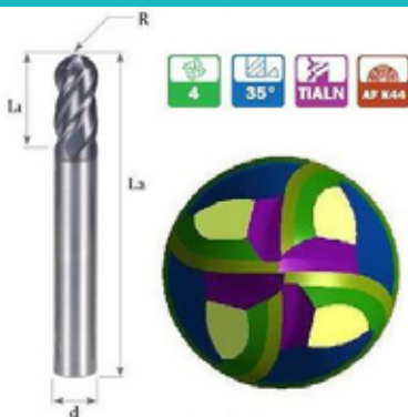
End mills
