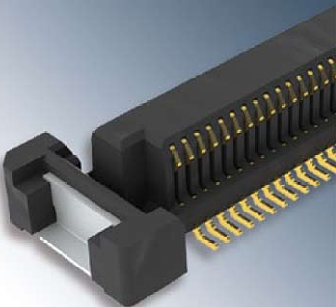
COM Express® 0.5 mm SMT Board-to-Board Connector
