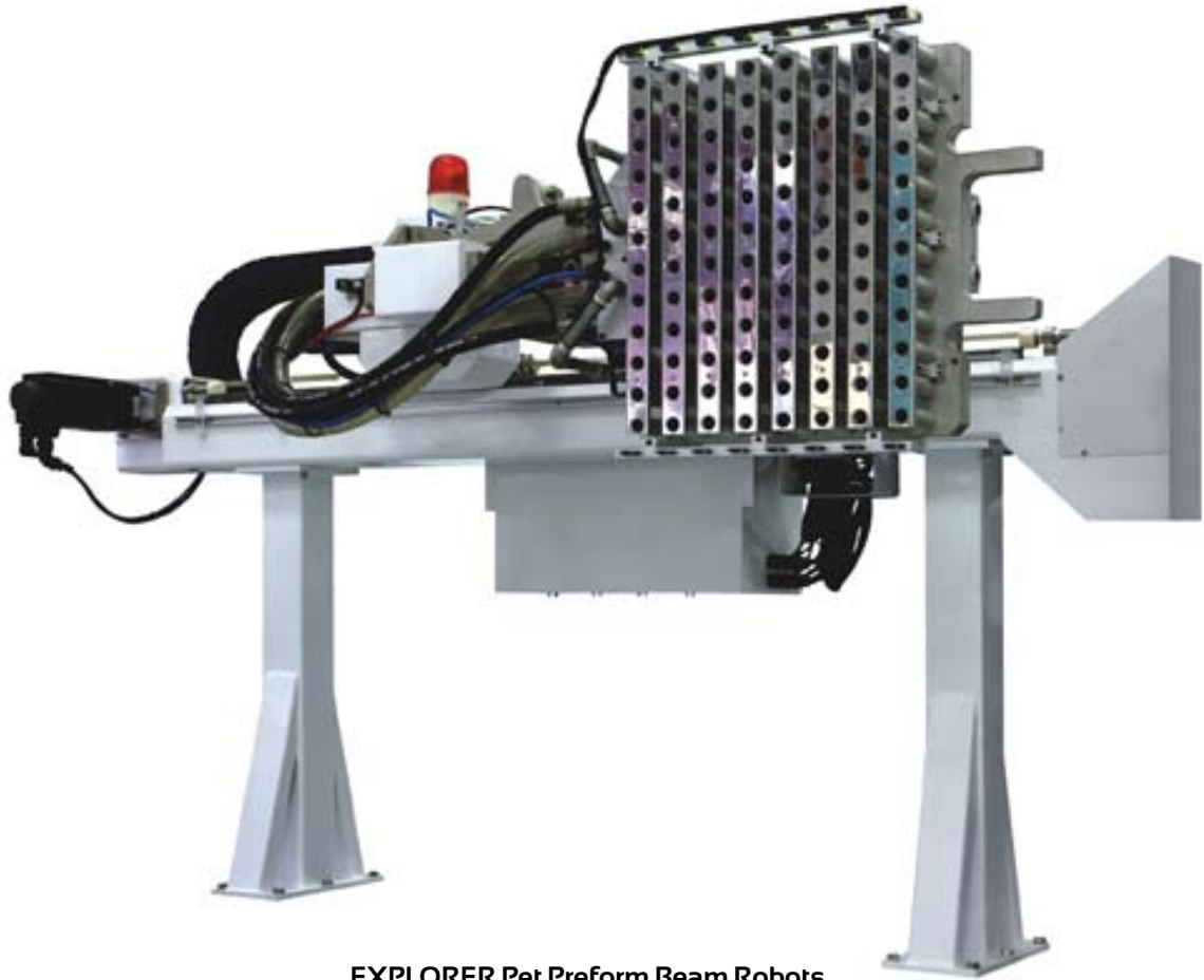
EXPLORER Pet Preform Beam Robots
