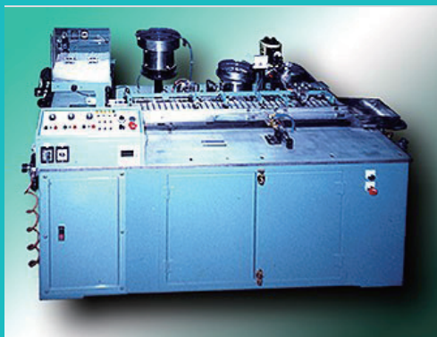
Gel Pen Refill Filling & Assembly Machine
