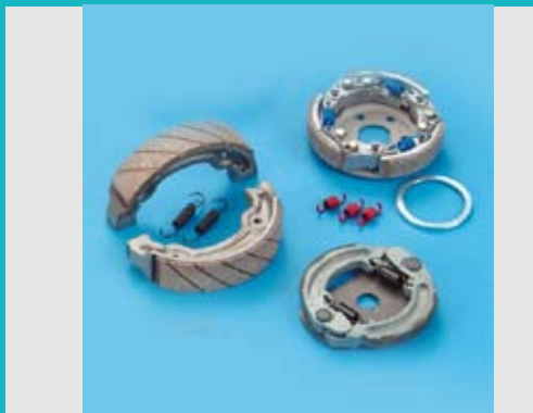
Brake Shoe
