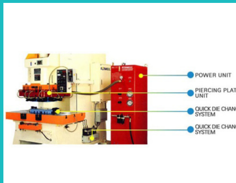
PCB Fine Piercing System
