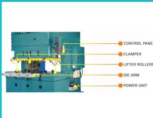
QUICK DIE CHANGE SYSTEM
