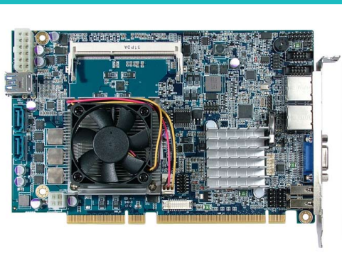
BH-0927 PICMG 1.3
