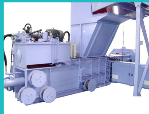
Automatic Horizontal Baling Press
