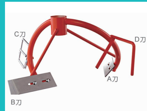
Mixer Arm
