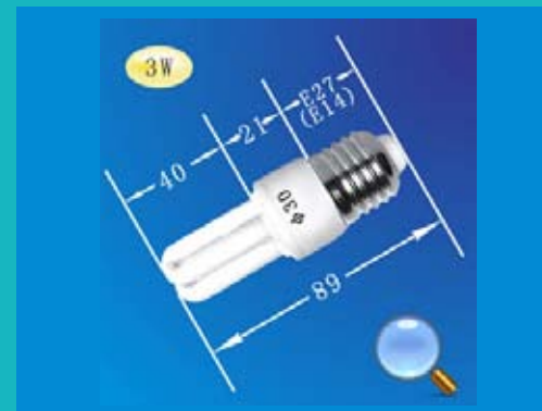
Electronic Energy-saving Lamp: 30 Series: T2 2U 30 3W/5W/8W/10W
